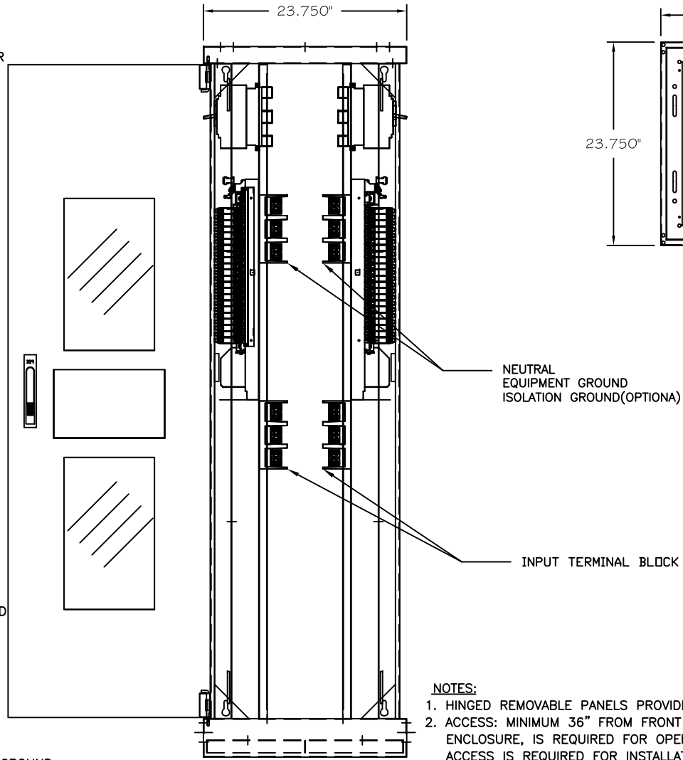
SIDE VIEW (DOOR & COVERS REMOVED)
