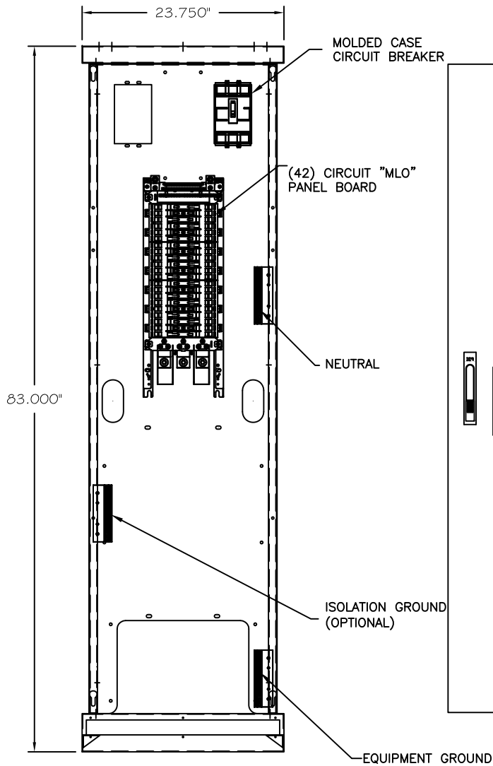
FRONT VIEW (DOOR & COVERS REMOVED)
