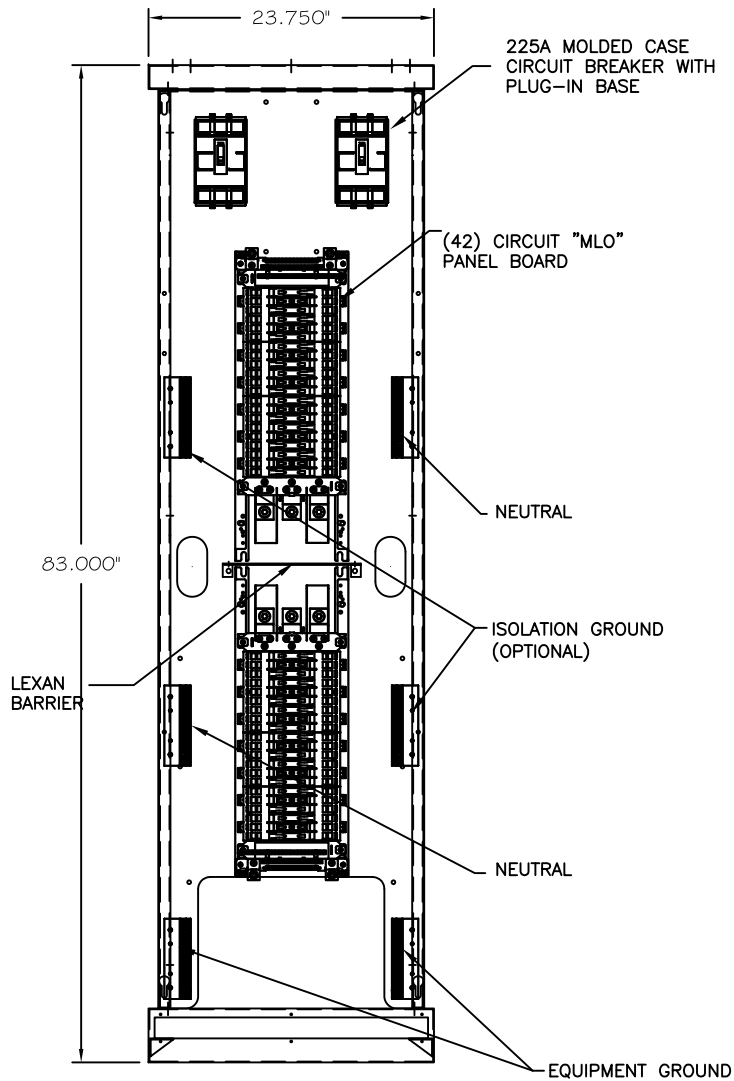
FRONT VIEW (DOOR & COVERS REMOVED)
