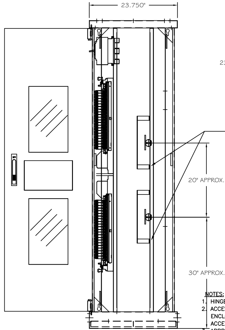
SIDE VIEW (DOOR & COVERS REMOVED)
