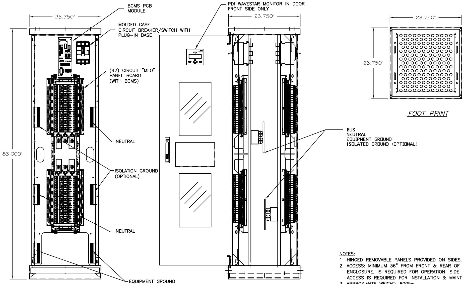
FRONT AND REAR VIEW (DOOR & COVERS REMOVED)
