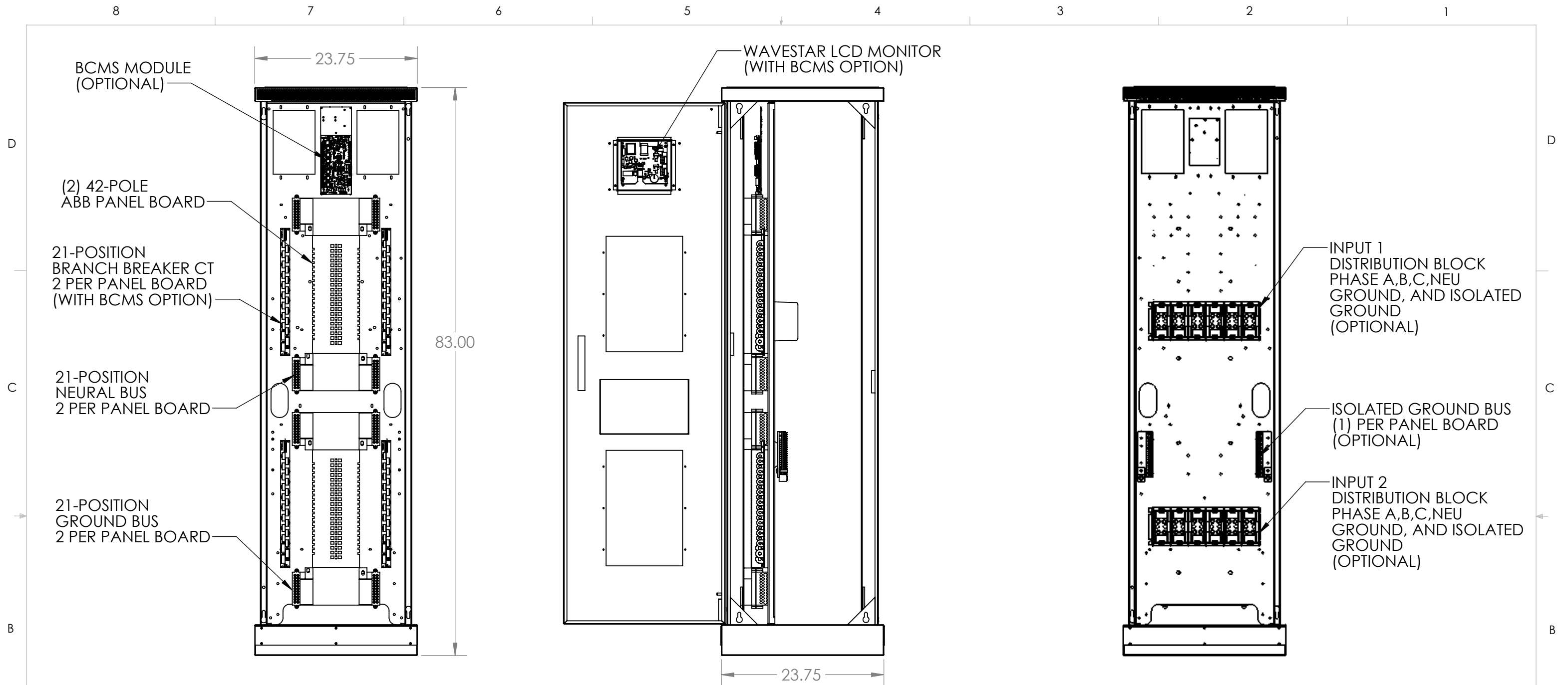
FRONT VIEW DOOR AND PANELS REMOVED
