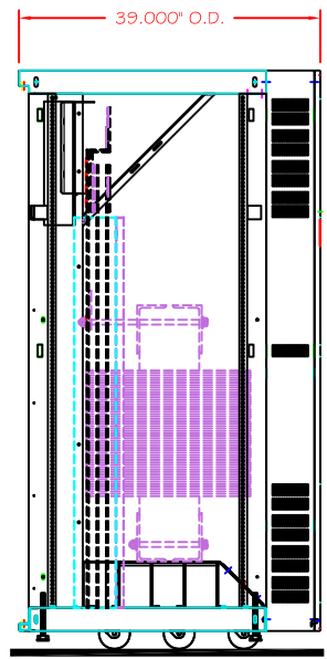
RIGHT SIDE VIEW (DOOR AND COVERS REMOVED)
