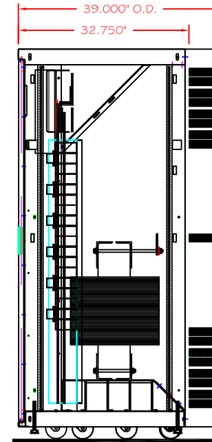
RIGHT SIDE VIEW (DOOR AND COVERS REMOVED)
