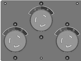
L6-20R
