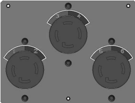
L14-30R
