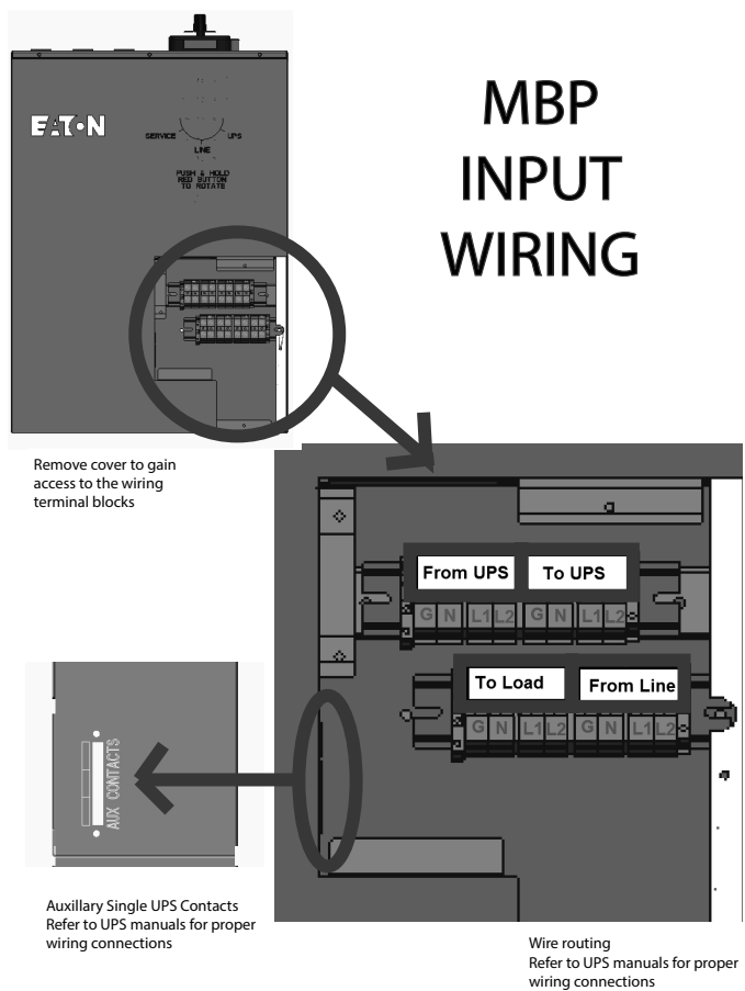
Figure 13. BPM Hardwired Overview
