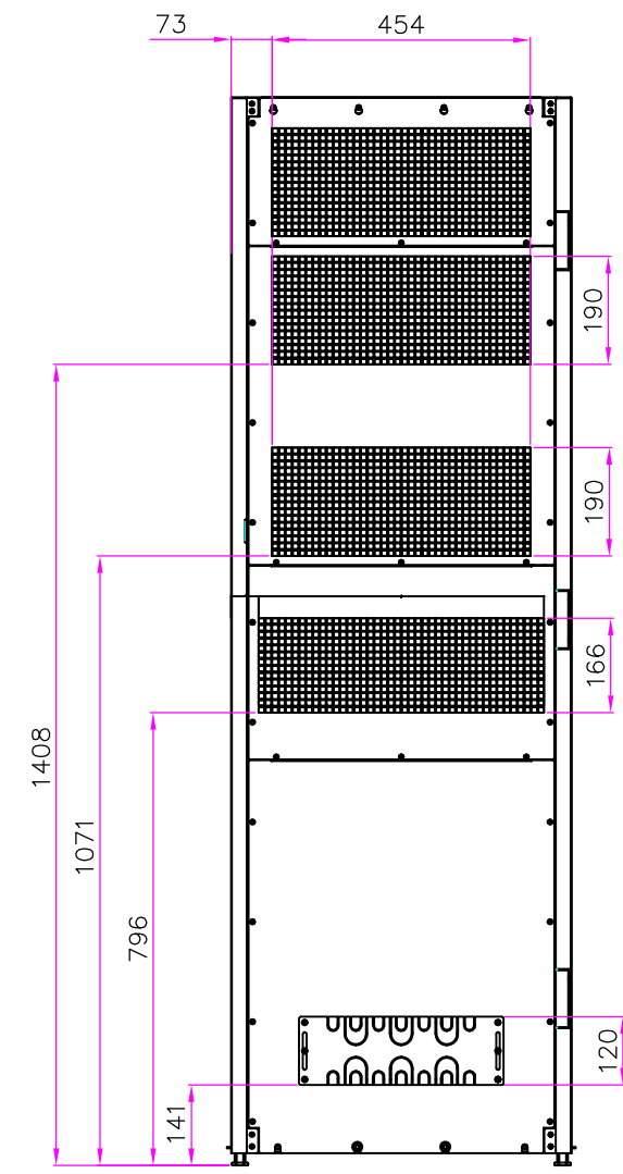
REAR VIEW
