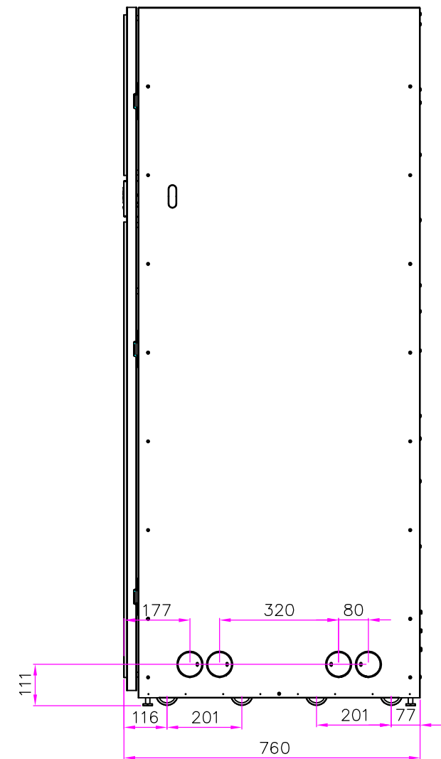
RIGHT VIEW
