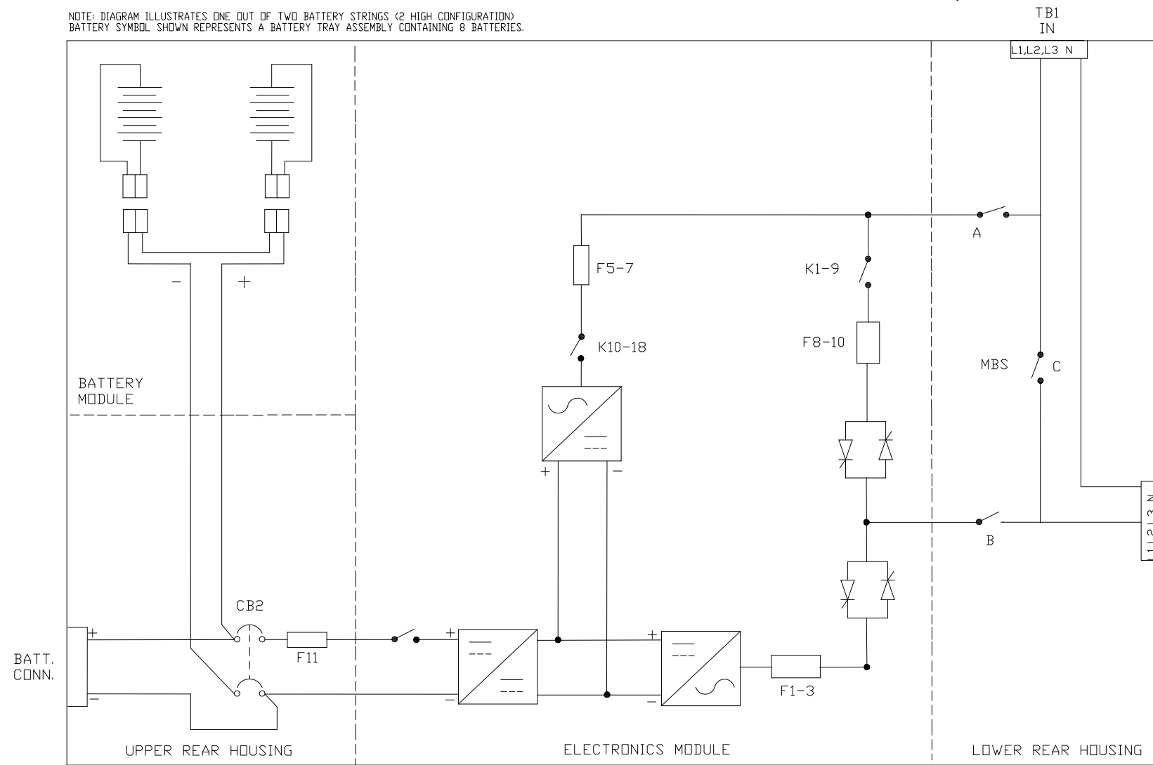
ONE LINE DIAGRAM FOR 9355 8-15KVA 2 HIGH UPS WITH INTERNAL BATTERIES
