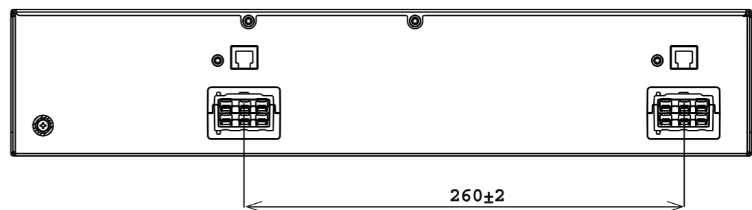
Rear Panel View
