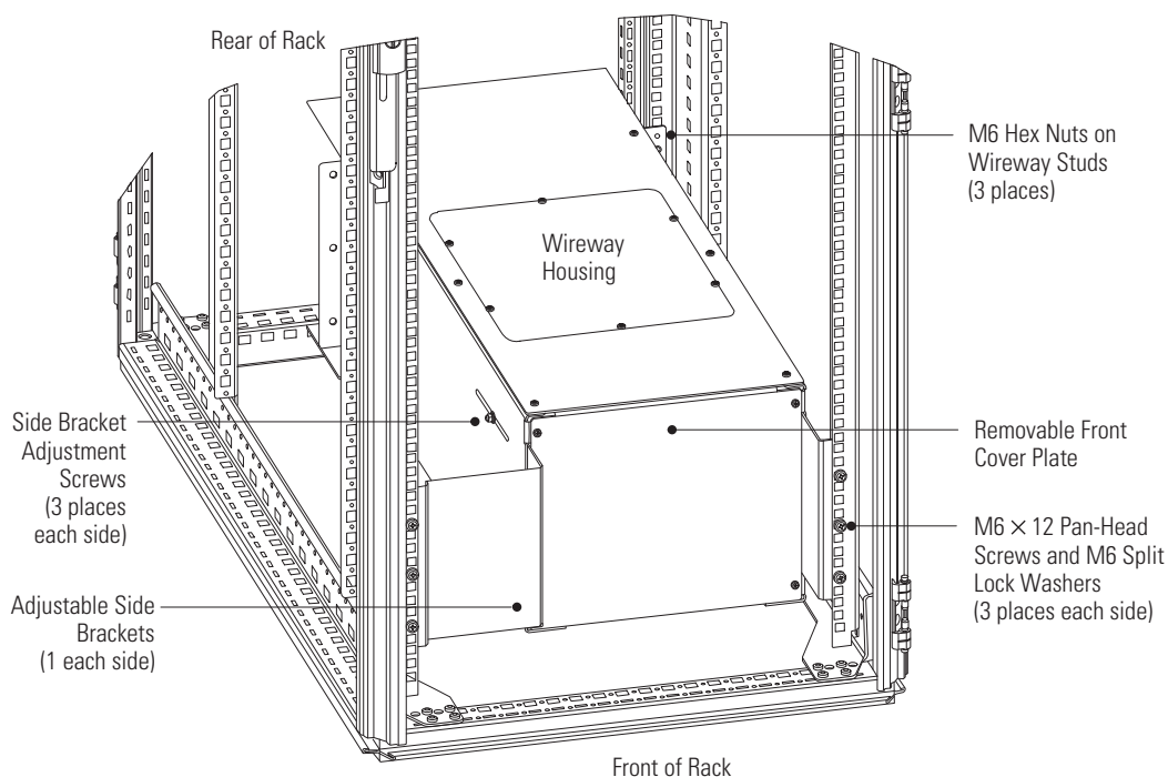
Figure 3. Wireway Installation
