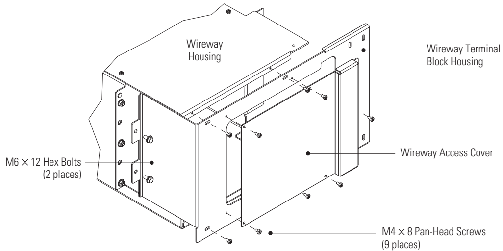
Figure 12. Wireway Disassembly
