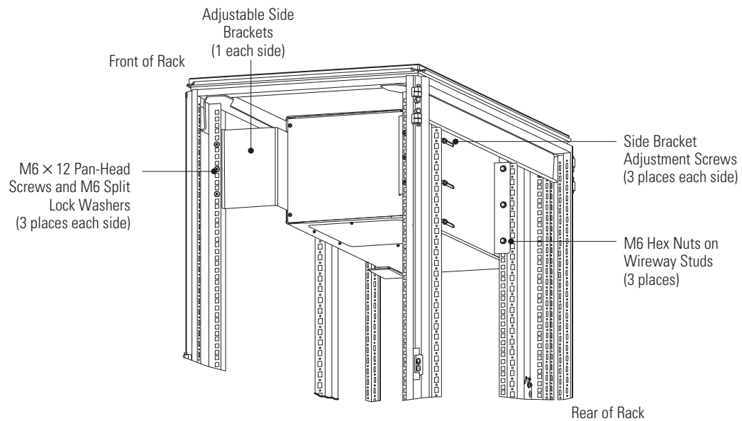
Figure 13. Wireway Installation
