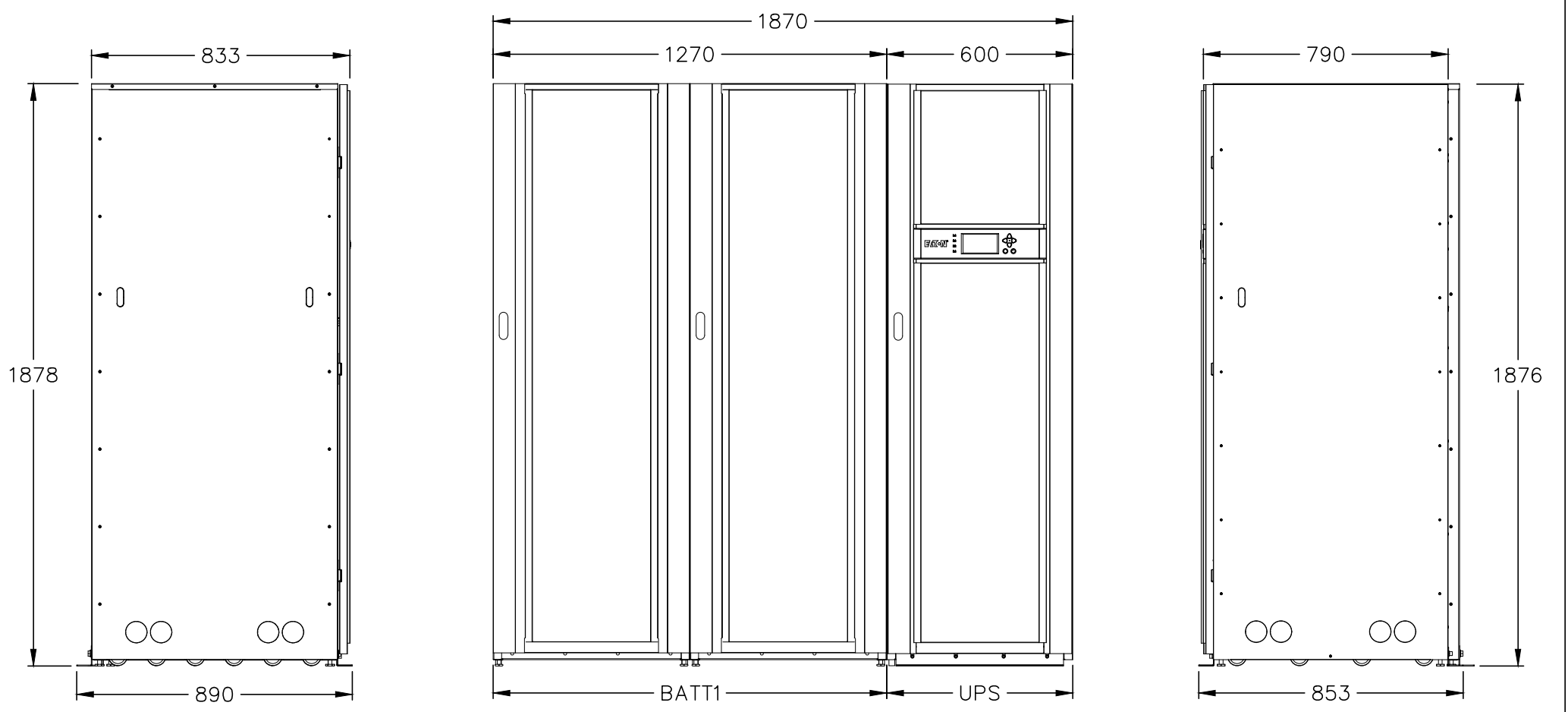
LEFT SIDE VIEW
