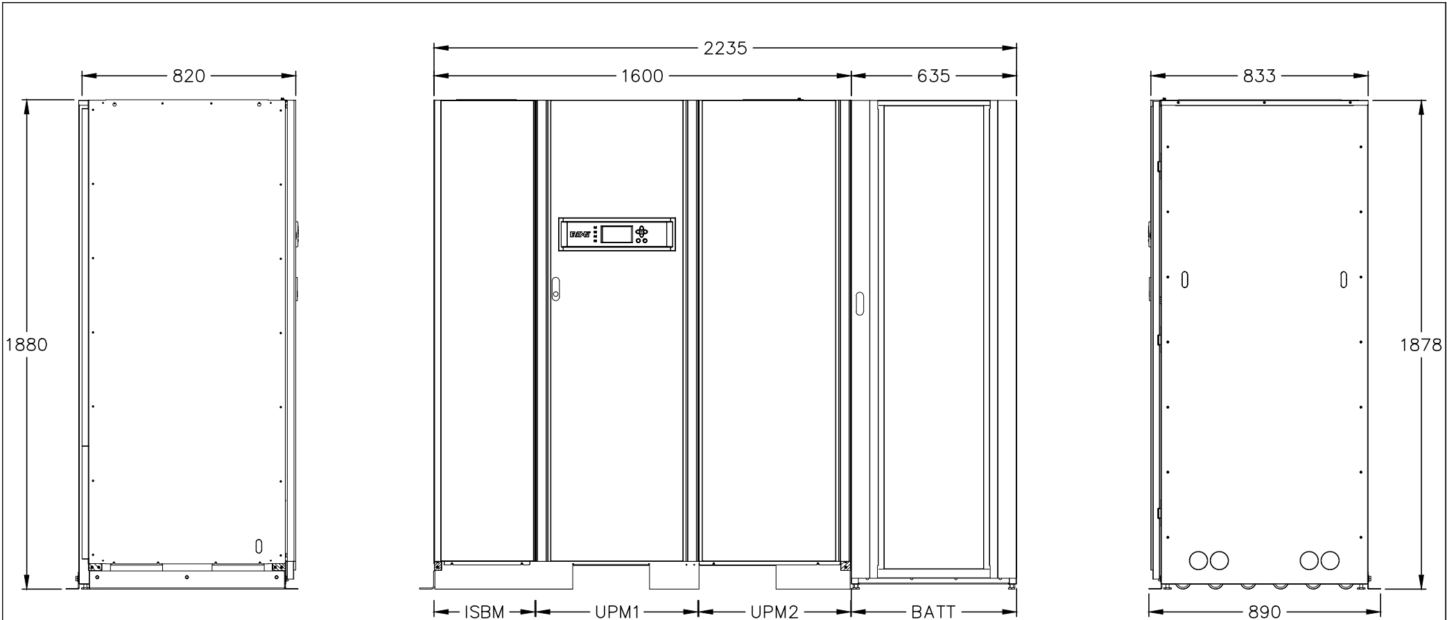
LEFT SIDE VIEW
