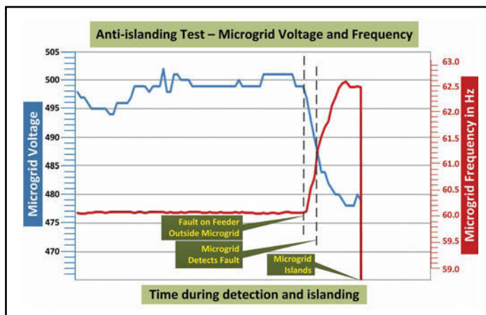
Figure 1. Anti-Islanding Test—Microgrid Voltage and Frequency
