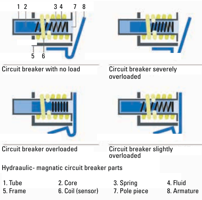
Figure 1. Hydraulic-magnetic circuit breaker principle
