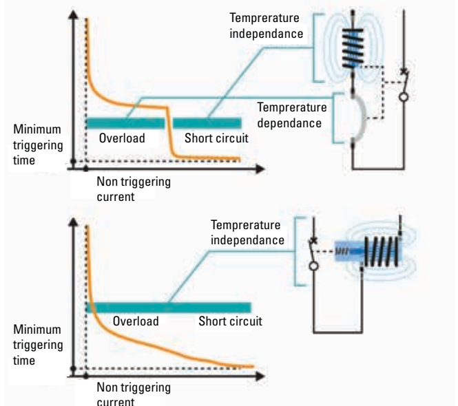
Figure 2. Comparison of trip mechanisms and response curves of thermo-magnetic vs hydraulic-magnetic breaker technology
