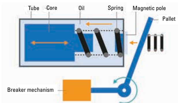
Figure 3. Mechanical arrangement of hydraulic-magnetic device, showing inbuilt resistance to physical shock and vibration
