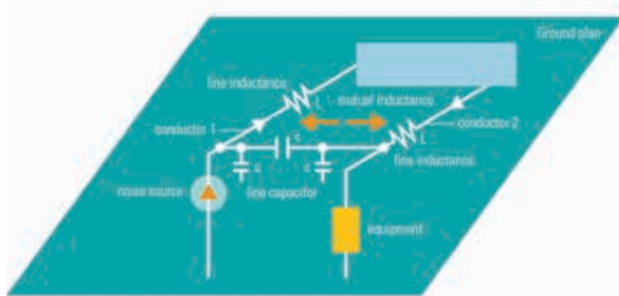
Figure 5. Long wire field schematic
