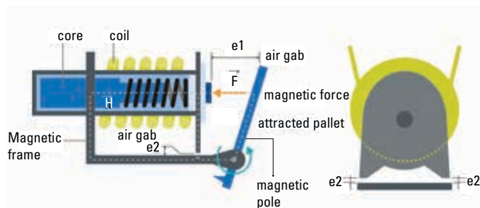
Figure 4. Role of air gaps in absorbing transient energy
