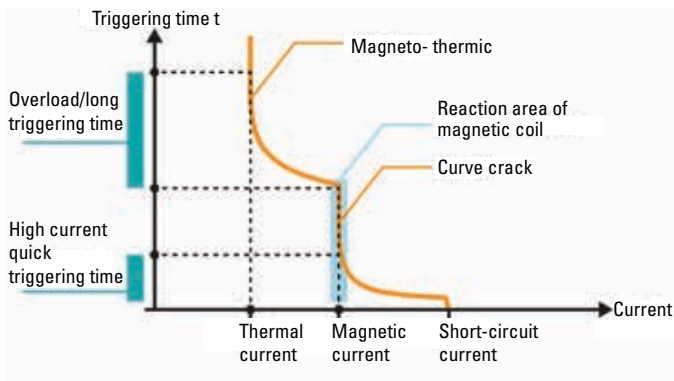
Figure 6. Showing sudden sharp decrease in triggering time at start of magnetic region
