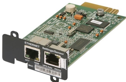
Figura 23. Scheda NETWORK-MS
