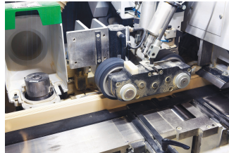
Feed rollers transport the wood through the machine, where it is processed with special tools (such as planers) into the required form
